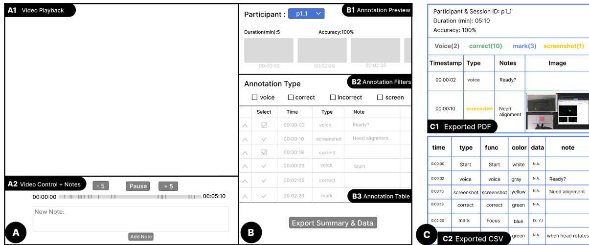
Fig. 5. The Analyzer interface comprises two main panels: the video panel (A) and the annotation panel (B). The video panel includes video playbacks of the pilot (A1), video controls, and a new note panel (A2). The annotation panel features an annotation preview (B1), annotation filtering options (B2), an annotation table (B3), and an exporting button. The Analyzer supports exporting the annotations (C) in PDF format (C1) and CSV format (C2).
